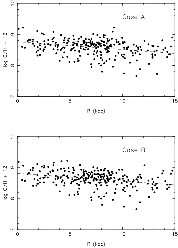
Fig. 2. Variation of oxygen abundance according to galactocentric distance of the whole sample; Cases A and B.
