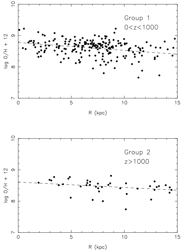
Fig. 4. The same as Figure 2, using 2 height groups with \Delta = 1,000 pc, Case A.
