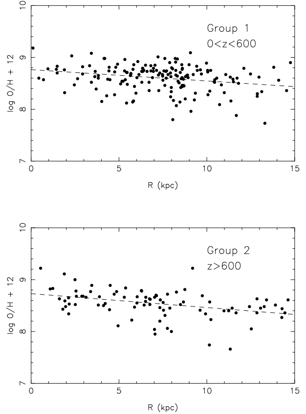
Fig. 6. The same as Figure 2, considering 2 height groups with \Delta = 600 pc, Case A.
