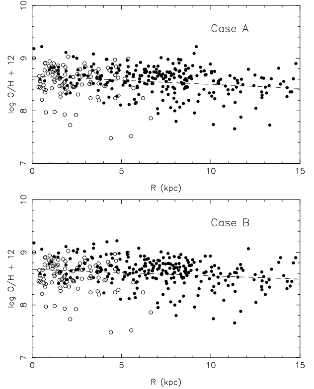
Fig. 7. The same as Figure 2, including objects from the bulge/disk interface region.
