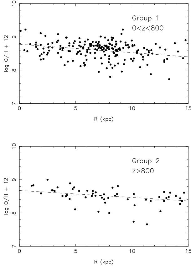
Fig. 5. The same as Figure 2, using 2 height groups with \Delta = 800 pc, Case A.
