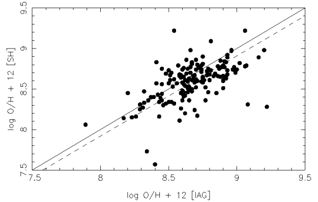
Fig. 1. Comparison of the oxygen abundances found by Stanghellini & Haywood (2010) ( y axis) and the abundances estimated from the IAG sample ( x axis).
