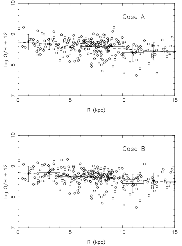
Fig. 3. The same as Figure 2, adopting average abundances in 2 kpc bins.
