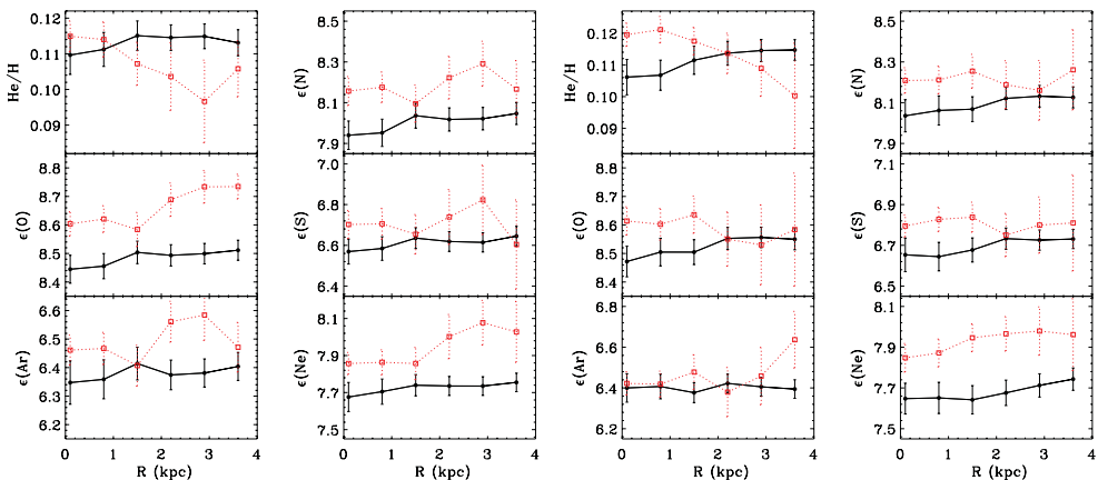
Figure 1. Average radial distribution of PNe chemical abundances based on (left) the Stanghellini et al. (2008; SSV08) and (right) the Zhang (1995; Z95) distance scales. Black solid circles represent group I and red open squares represent group II PNe. For the Z95 scale, R is given as R_L .
