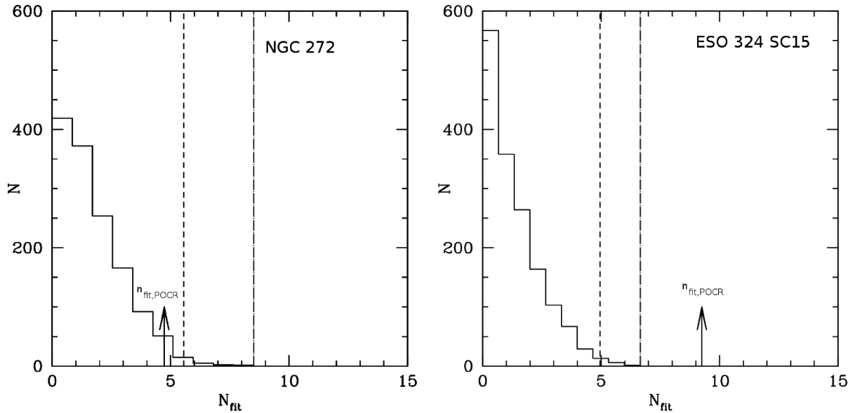
Figure 10. Number of isochrone-fitted stars weighted by membership probability for the neighbouring sample fields ( n_{\text{fit}} – histogram) and the targets ( n_{\text{fit,POCR}} – arrow), but for the surrounding control field radius 60 arcmin. The percentile locus 99 per cent and n_{\text{fit,lim}} are marked (vertical dashed lines).
