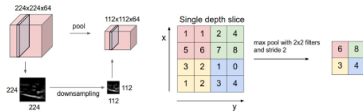
Figure : Left: Pooling, right: max pooling example
