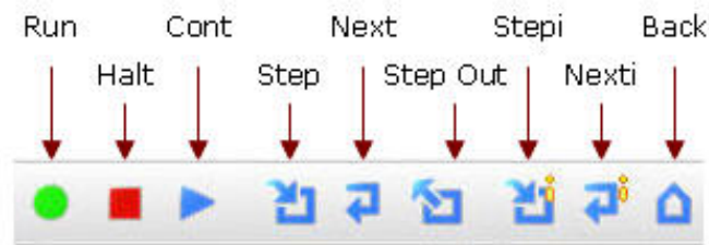
Figure 2.6. PGDBG Toolbar
