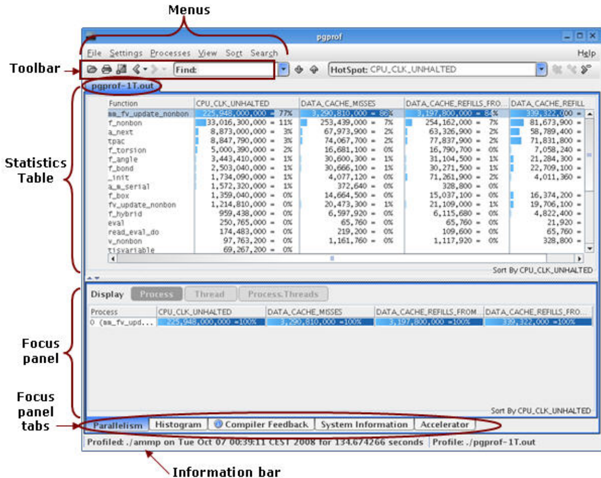
Figure 15.1. PGPROF Overview
