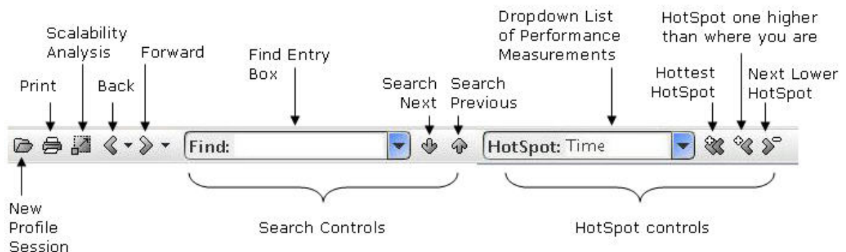
Figure 20.7. PGPROF Toolbar
