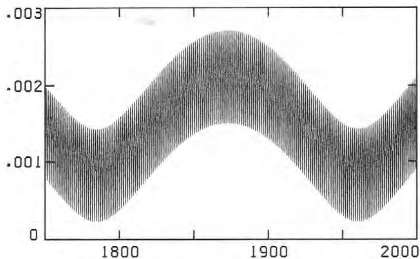
FIGURE 6.1 - ECCENTRICITY OF J3(GANYMEDE)
