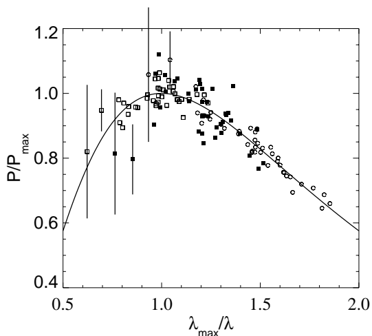
Fig. 4. The normalized wavelength dependence of the interstellar linear polarization derived from the 40 stars showing degree of polarization greater than 0.5% in all the observed passbands. The solid line represents the Serkowski's empirical formula relating the ratio P/P_{\max} to the corresponding ratio \lambda_{\max}/\lambda . The bars indicate the observed uncertainties for HD 79936 and HD 80085 (see text). The U , B , and V colours are represented by open circles, filled squares and open squares, respectively
