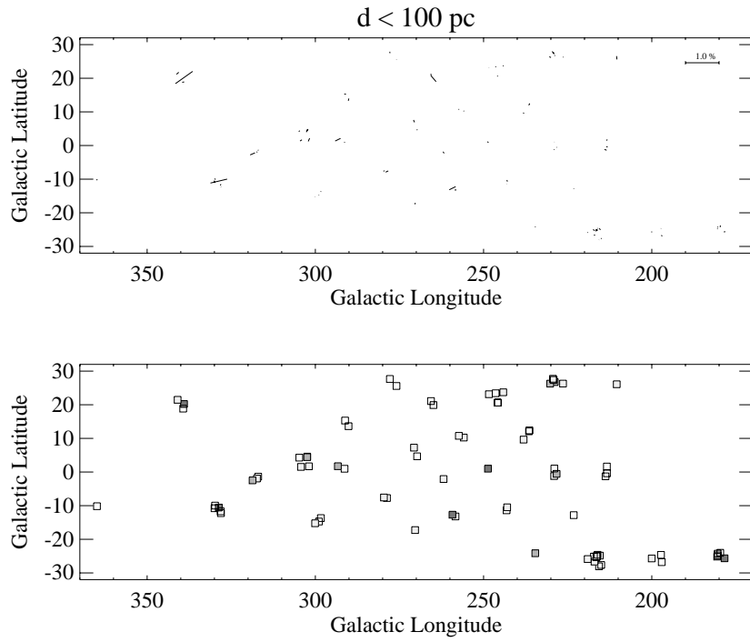
Fig. 8. Observed polarization ( B -band) and colour excess E(b - y) up to 100 pc. The estimated colour excess are indicated by the small squares as: (□) E(b - y) < 0^m017 . (◻) 0^m017 \leq E(b - y) < 0^m030 . (◼) 0^m030 \leq E(b - y) < 0^m050 . (■) 0^m050 \leq E(b - y) < 0^m100 . (■) 0^m100 \leq E(b - y) < 0^m200 . (■) E(b - y) \geq 0^m200
