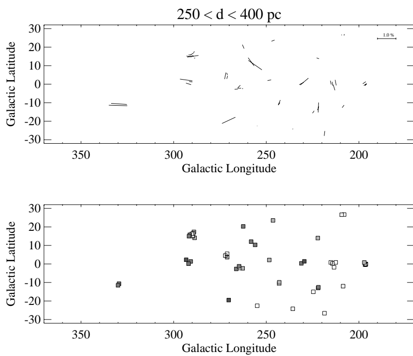
Fig. 11. Same as Fig. 8. Stars in the range 250 \leq d < 400 pc
