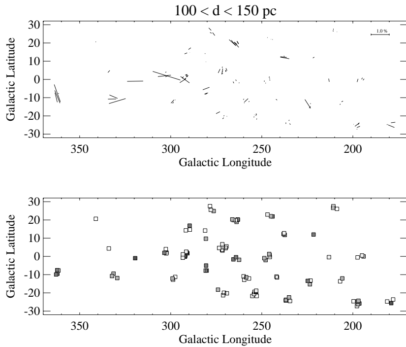
Fig. 9. Same as Fig. 8. Stars in the range 100 \leq d < 150 pc
