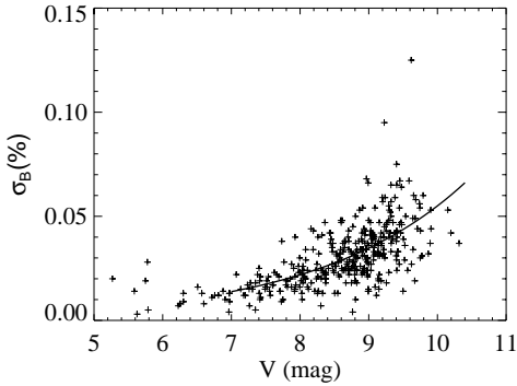
Fig. 2. Estimated error in the B -band versus stellar visual magnitude. The errors of bright stars ( V \lesssim 7^m0 ) are mainly dominated by atmospheric scintillation. For fainter stars, it is dominated by photon shot noise and, in the present case, may be roughly represented by \sigma_B = 5.5 \cdot 10^{-4} (10^V)^{1/5} (solid curve)
