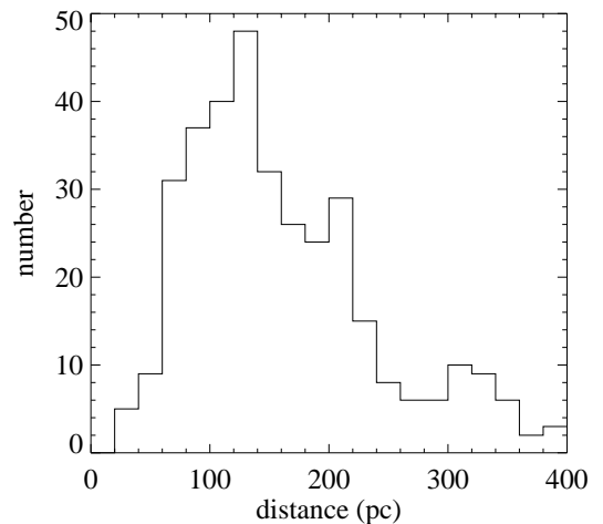
Fig. 3. The distribution of the observed stars as a function of the distance. Nineteen stars are located beyond the distance interval represented in this histogram
