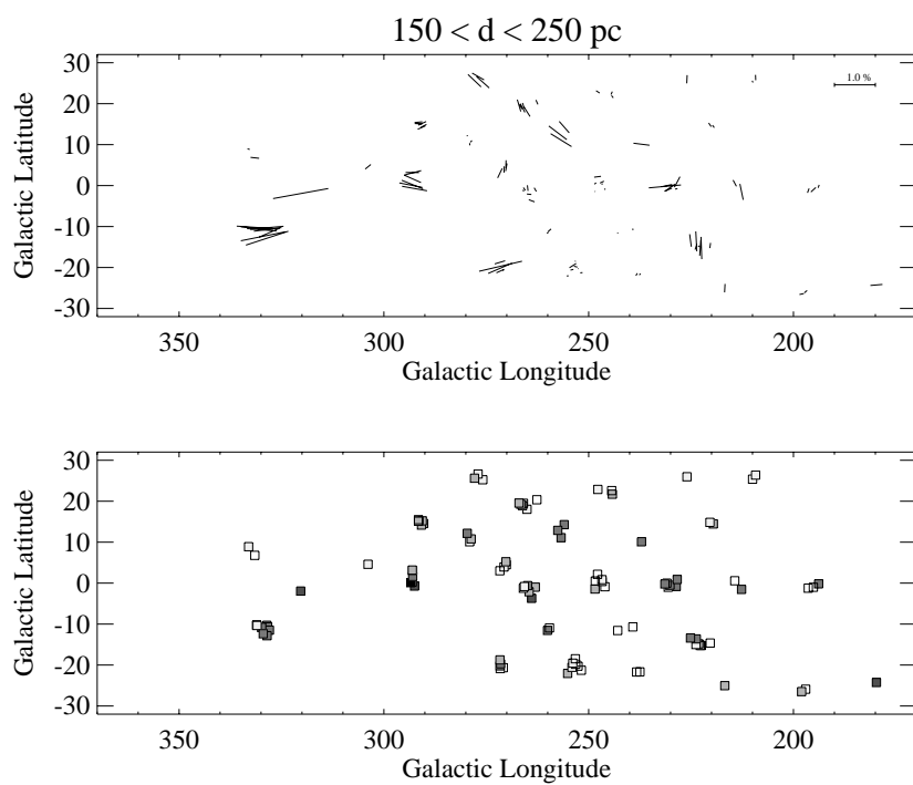
Fig. 10. Same as Fig. 8. Stars in the range 150 \leq d < 250 pc
