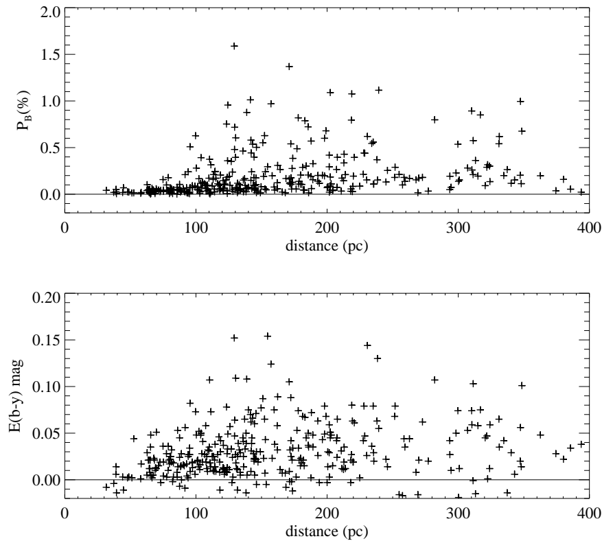
Fig. 7. ( upper ) The polarization in the B -band versus distance. ( lower ) E(b - y) versus distance. Although polarization is a positive quantity, the vertical axis of the upper diagram has been extended to negative values in order to make easier the comparison between both diagrams. It is remarkable, nevertheless the positive bias, the small degree of the observed linear polarization showed by stars up to \approx 100 pc
