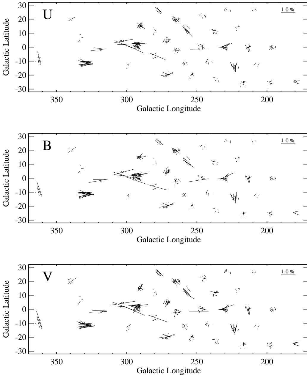
Fig. 1. The E -vectors of the UBV polarization measurements. The length of each line is proportional to P , the percentage polarization and the angle at which each line is drawn relative to the galactic north pole in the direction of increasing longitude is \theta_{\text{gal}}
