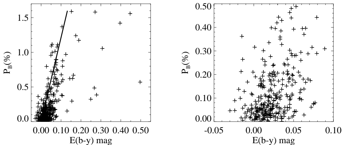
Fig. 6. The polarization in the B -band versus E(b-y) . ( left ) All observed stars. The solid line represents optimum alignment efficiency ( P(\%) = 12.1 \times E(b-y) ; E(b-y) = 0.74 E(B-V) ). ( right ) Expanded view for the low reddening part of the diagram
