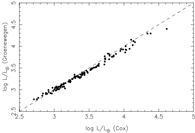
Fig. 6. A comparison of the luminosities calculated using Method 1 (Eq. (4)) from Cox (2000) and Method 2 (Eq. (7)) from Groenewegen et al. (2004).
