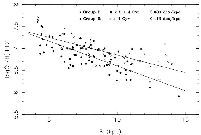
Fig. 3. The S/H abundance gradient from planetary nebulae, divided into two age groups: Group I ( t < 4 Gyr, empty circles) and Group II ( t > 4 Gyr, filled circles). The corresponding gradients (dex/kpc) are shown in the figure. The adopted value of the galactocentric distance of the Sun is R_0 = 8.0 kpc.
