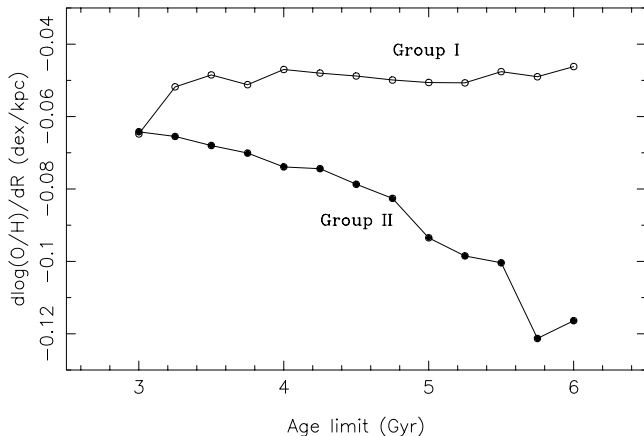
Fig. 1. Time variation of the O/H gradient from planetary nebulae. The PN sample was divided into two age groups, Group I (“younger”), with ages lower than the age limit t_1 , and Group II (“older”), with ages higher than t_1 . The plot shows the O/H gradient (dex/kpc) of each group as a function of the upper age limit of Group I, t_1 . The gradients of the younger Group I (open circles connected by lines) are always flatter than those of the older Group II (filled circles connected by lines). The best results apply for t_1 \simeq 4 to 5 Gyr, approximately, for which the correlations are more meaningful.
