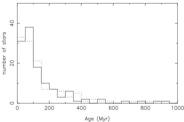
Fig. 7. A comparison of the age distributions of cepheid variables using ages from Bahcall & Piran (1983) (solid line, see Eq. (5)) and Binney & Merrifield (1998) (dotted line, see Eq. (6)). The period-luminosity relation is from Groenewegen et al. (2004), (see Eq. (7)).
