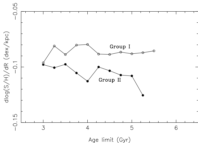
Fig. 2. The S/H gradient (dex/kpc) from planetary nebulae, divided into two age groups, as a function of the upper age limit of Group I. The gradients of the younger Group I (open circles connected by lines) are always flatter than those of the older Group II (filled circles connected by lines).
