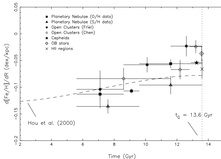
Fig. 8. Time variation of the [\text{Fe}/\text{H}] abundance gradient (dex/kpc). The converted [\text{Fe}/\text{H}] gradients from planetary nebulae are shown as filled squares (O/H data) and filled triangles (S/H data). The open cluster results are shown as filled circles (data from Friel et al. 2002) and empty circles (data from Chen et al. 2003). The [\text{Fe}/\text{H}] gradient from cepheid variables is shown as a filled star. Also included are the following young objects: OB stars in associations etc. from Daflon & Cunha (2004, thick cross) and HII regions (x sign). The dotted vertical line shows the adopted age of the galactic disk, t_G = 13.6 Gyr, and the dashed line represents the time evolution of the [\text{Fe}/\text{H}] gradient according to the theoretical models of Hou et al. (2000).
