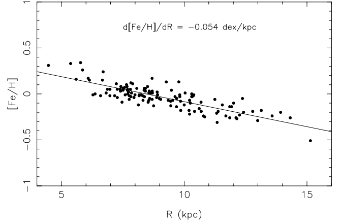
Fig. 5. The [\text{Fe}/\text{H}] abundance gradient from cepheid variable stars. The correlation coefficient is r = -0.82 , and a total of 127 stars have been included. The adopted value for the galactocentric distance of the Sun is R_0 = 8.0 kpc.
