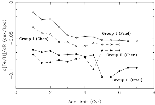
Fig. 4. The [\text{Fe}/\text{H}] gradient (dex/kpc) from the samples of open clusters by Friel et al. (2002, solid lines), and Chen et al. (2003, dashed lines), divided into two age groups, as a function of the upper age limit of Group I. As for the case of planetary nebulae, the gradients of the younger Group I (open circles) are always flatter than those of the older Group II (filled circles).
