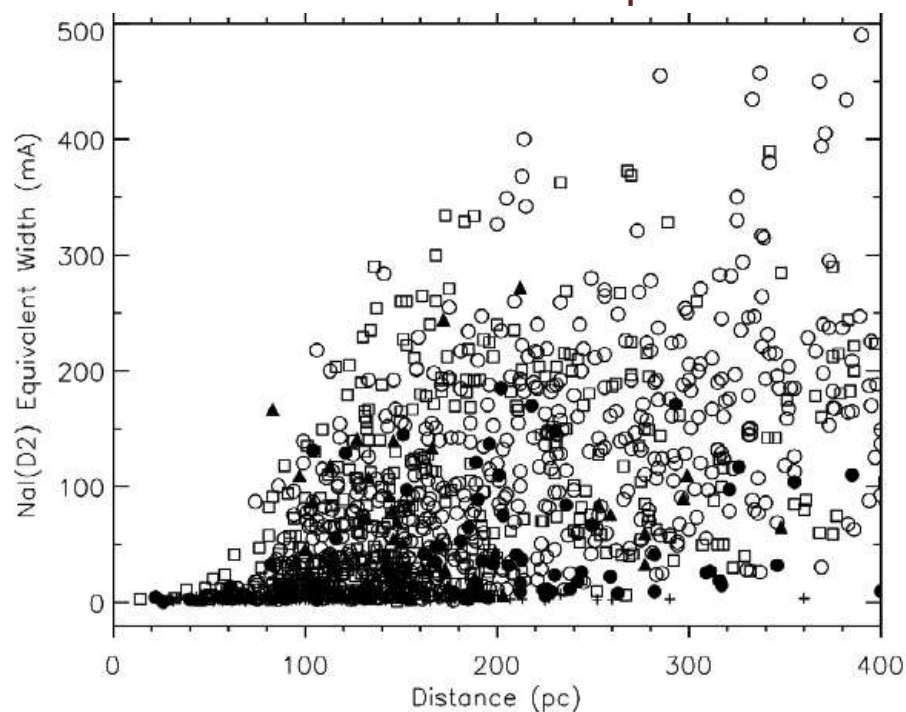
Fig. 7. Plot of the equivalent width ( m\text{\AA} ) of the interstellar NaI D2-line for stars with distances <400 pc. Filled triangles are for sight-lines with galactic latitude b > +45^\circ , open squares for sight-lines with b = 0 to 45^\circ , open circles for sight-lines with b = 0 to -45^\circ and filled circles for sight-lines with b < -45^\circ . Crosses are upper limit values. Note the sharp increase in the level of NaI absorption at \sim 80 pc, which is due to the neutral wall to the Local Cavity.
