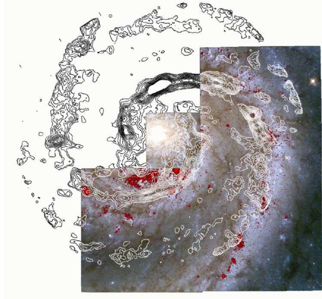
M51: CO contours overlaid on Pa emission + optical
