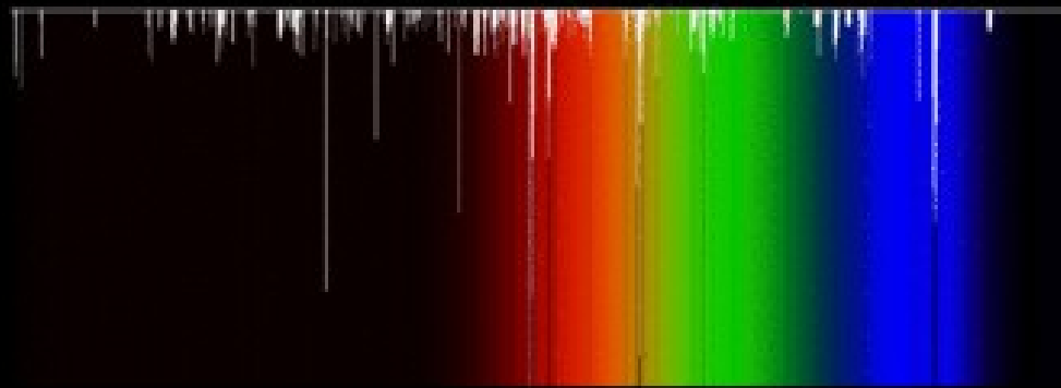
The Diffuse Interstellar Bands
